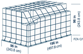
IATA ULD code: PZA Q7 Universal general-purpose flat pallet for lower holds and main decks.
