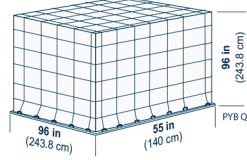
IATA ULD code: PYB Q6 Universal general-purpose flat pallet for lower holds and main decks.
